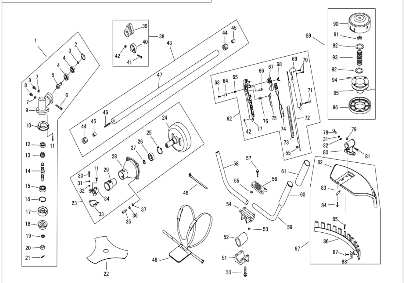
FIG. 2: CG520B-CE SHOULDER BRUSH CUTTER
