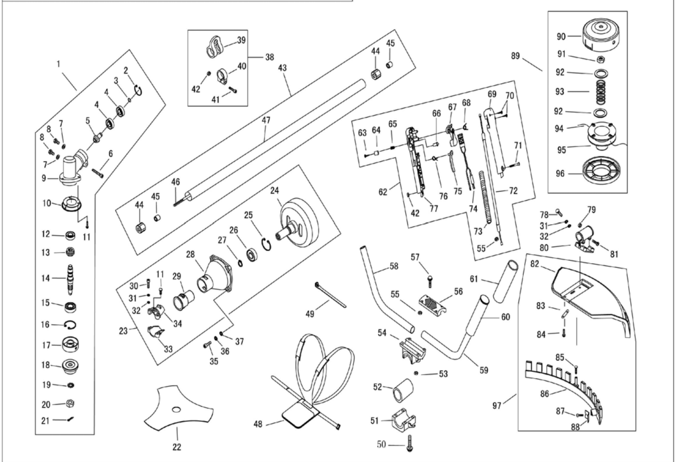
FIG. 2: CG520B-CE SHOULDER BRUSH CUTTER
